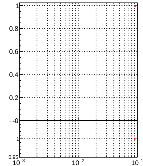
- /data2/legianni/BDT-vs-DNN/real-BDT/CMSSW_13_0_0_pre4/src/runrem/DQM_TT_mkFit_ - DQM_TT_mkFitRETEST_
