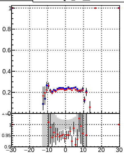
/data2/legianni/BDT-vs-DNN/real-BDT/CMSSW_13_0_0_pre4/src/runrem/DQM_TT_mkFit_ DQM_TT_mkFitRETEST_ Fake rate vs vertpos
