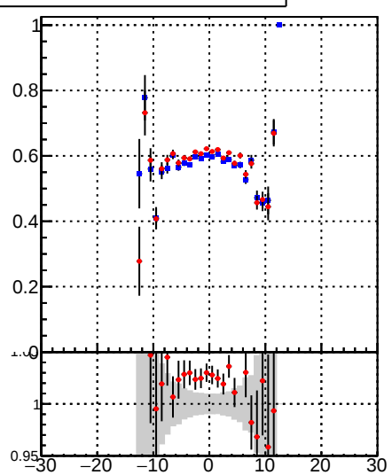
/data2/legianni/BDT-vs-DNN/real-BDT/CMSSW_13_0_0_pre4/src/runrem/DQM_TT_mkFit_ DQM_TT_mkFitRETEST_ Pileup rate vs vertpos
