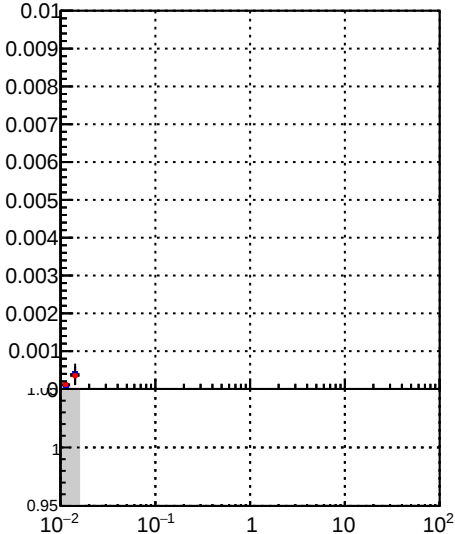
/data2/legianni/BDT-vs-DNN/real-BDT/CMSSW_13_0_0_pre4/src/runrem/DQM_TT_mkFit_ DQM_TT_mkFitRETEST_ Duplicates Rate vs vertpos
