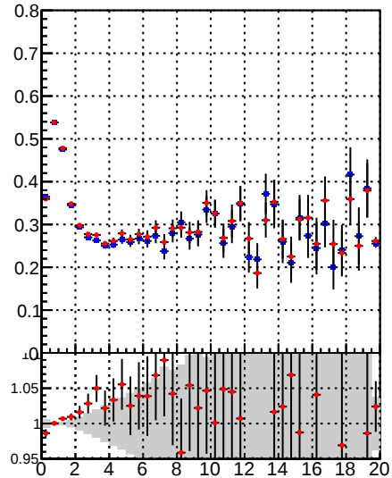
Purity rate vs normalized \chi^2
