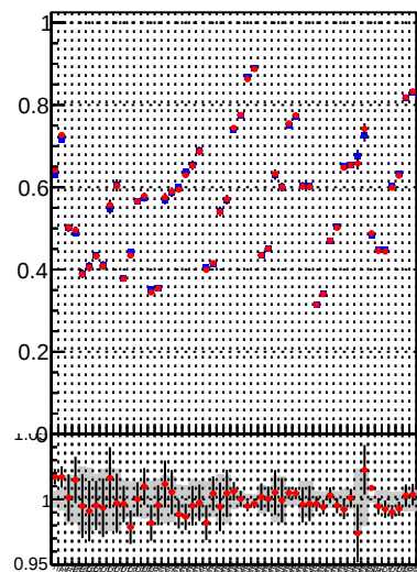
Fake rate vs. — /data2/legianni/BDT-vs-DNN/real-BDT/CMSSW_13_0_0_pre4/src/runrem/DQM_TT_mkFit_ — DQM_TT_mkFitRETEST
