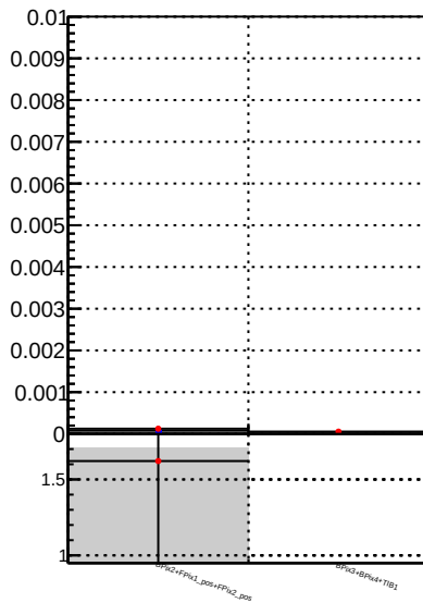
— /data2/legianni/BDT-vs-DNN/real-BDT/CMSSW_13_0_0_pre4/src/runrem/DQM_TT_mkFit_ — DQM_TT_mkFitRETEST
