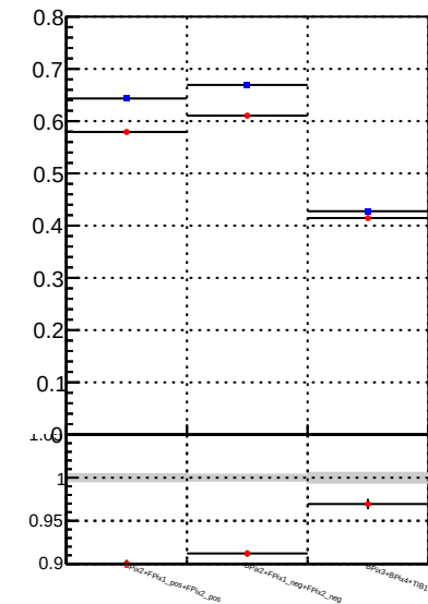
— /data2/legianni/BDT-vs-DNN/real-BDT/CMSSW_13_0_0_pre4/src/runrem/DQM_TT_mkFit_ — DQM_TT_mkFitRETEST
