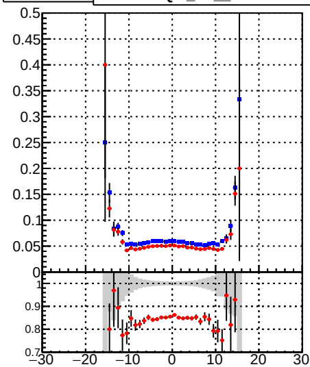
/data2/legianni/BDT-vs-DNN/real-BDT/CMSSW_13_0_0_pre4/src/runrem/DQM_TT_mkFit_ DQM_TT_mkFitRETEST_ Fake rate vs vertpos
