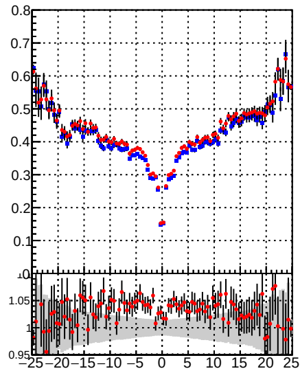
—•— /data2/legianni/BDT-vs-DNN/real-BDT/CMSSW_13_0_0_pre4/src/runrem/DQM_TT_mkFit_ —•— DQM_TT_mkFitRETEST
