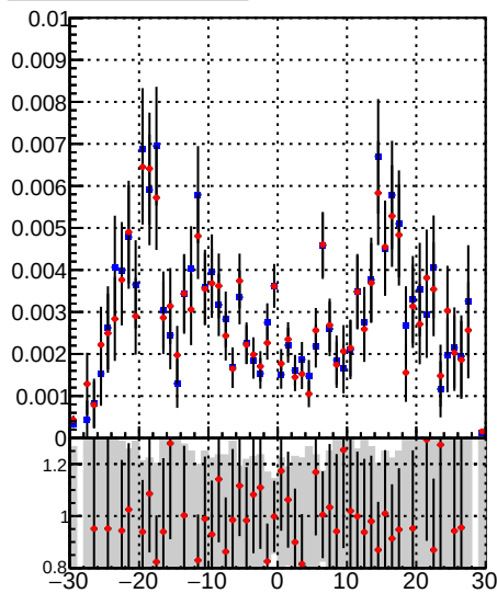
—•— /data2/legianni/BDT-vs-DNN/real-BDT/CMSSW_13_0_0_pre4/src/runrem/DQM_TT_mkFit_ —•— DQM_TT_mkFitRETEST
