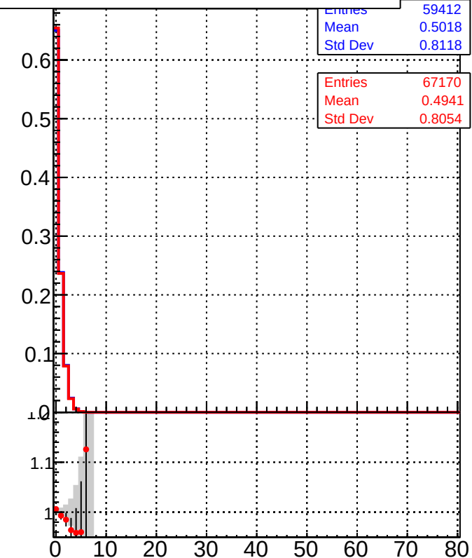
/data2/legianni/BDT-vs-DNN/real-BDT/CMSSW_13_0_0_pre4/src/runrem/DQM_TT_mkFit_ DQM_TT_mkFitRETEST_
