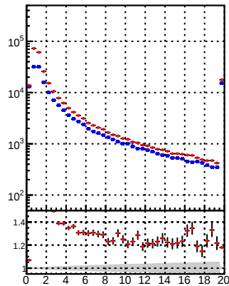
- /data2/legianni/BDT-vs-DNN/real-BDT/CMSSW_13_0_0_pre4/src/runrem/DQM_TT_mkFit - DQM_TT_mkFitRETEST_
