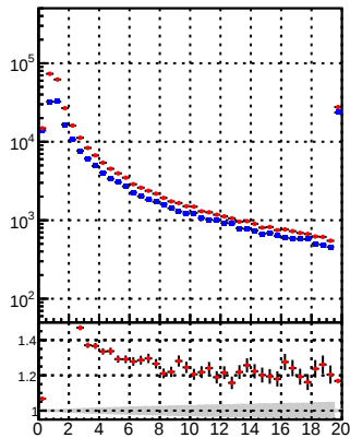
- /data2/legianni/BDT-vs-DNN/real-BDT/CMSSW_13_0_0_pre4/src/runrem/DQM_TT_mkFit - DQM_TT_mkFitRETEST_
