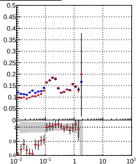
—•— /data2/legianni/BDT-vs-DNN/real-BDT/CMSSW_13_0_0_pre4/src/runrem/DQM_TT_mkFit_ —•— DQM_TT_mkFitRETEST_
