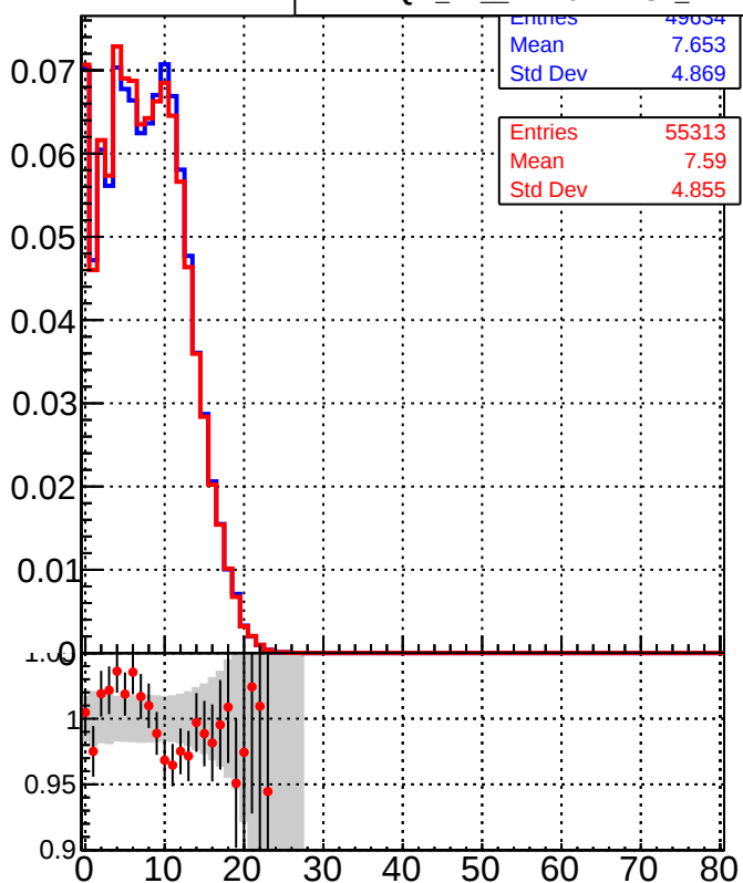
Legend for the bottom row of plots: —■— /data2/legianni/BDT-vs-DNN/real-BDT/CMSSW_13_0_0_pre4/src/runrem/DQM_TT_mkFit_ —●— DQM_TT_mkFitRETEST_
