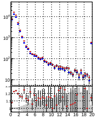
N of reco track vs. \chi^2 —•— /data2/legianni/BDT-vs-DNN/real-BDT/CMSSW_13_0_0_pre4/src/runrem/DQM_TT_mkFit —•— /data2/legianni/BDT-vs-DNN/real-BDT/CMSSW_13_0_0_pre4/src/runrem/DQM_TT_mkFitRETEST
