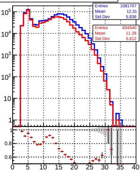
mean hit — /data2/legianni/BDT-vs-DNN/real-BDT/CMSSW_13_0_0_pre4/src/runrem/DQM_TT_mkFit_ — DQM_TT_mkFitRETEST_
