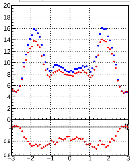
/data2/legianni/BDT-vs-DNN/real-BDT/CMSSW_13_0_0_pre4/src/runrem/DQM_TT_mkFit_ DQM_TT_mkFitRETEST_ mean hit
