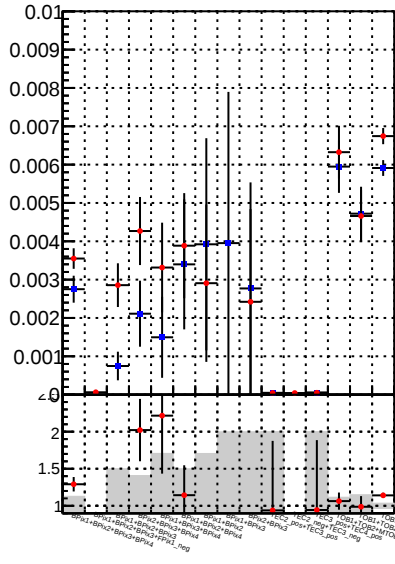
—●— /data2/legianni/BDT-vs-DNN/real-BDT/CMSSW_13_0_0_pre4/src/runrem/DQM_TT_mkFit_ —●— DQM_TT_mkFitRETEST
