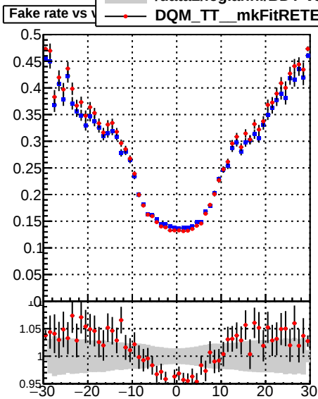
—•— /data2/legianni/BDT-vs-DNN/real-BDT/CMSSW_13_0_0_pre4/src/runrem/DQM_TT_mkFit_ —•— DQM_TT_mkFitRETEST_
