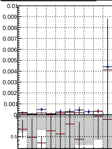
— /data2/legianni/BDT-vs-DNN/real-BDT/CMSSW_13_0_0_pre4/src/runrem/DQM_TT_mkFit_ — DQM_TT_mkFitRETEST
