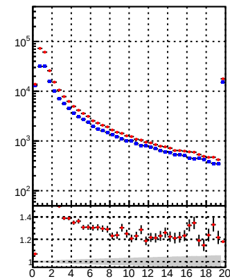
N of reco track vs. \chi^2 for /data2/legianni/BDT-vs-DNN/real-BDT/CMSSW_13_0_0_pre4/src/runrem/DQM_TT_mkFit vs /data2/legianni/BDT-vs-DNN/real-BDT/CMSSW_13_0_0_pre4/src/runrem/DQM_TT_mkFitRETEST
