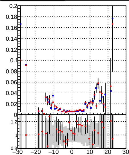
/data2/legianni/BDT-vs-DNN/real-BDT/CMSSW_13_0_0_pre4/src/runrem/DQM_TT_mkFit_ DQM_TT_mkFitRETEST
