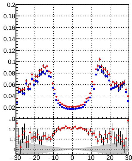
—•— /data2/legianni/BDT-vs-DNN/real-BDT/CMSSW_13_0_0_pre4/src/runrem/DQM_TT_mkFit_ —•— DQM_TT_mkFitRETEST
