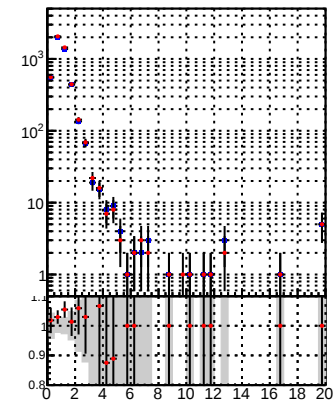
N of reco track vs. \chi^2 - \bullet /data2/legianni/BDT-vs-DNN/real-BDT/CMSSW_13_0_0_pre4/src/runrem/DQM_TT_mkFit - \bullet DQM_TT_mkFitRETEST
