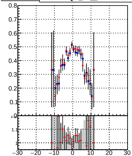
—●— /data2/legianni/BDT-vs-DNN/real-BDT/CMSSW_13_0_0_pre4/src/runrem/DQM_TT_mkFit_ —●— DQM_TT_mkFitRETEST_ Fake rate vs v
