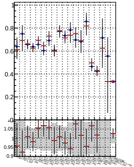
Fake rate vs. — /data2/legianni/BDT-vs-DNN/real-BDT/CMSSW_13_0_0_pre4/src/runrem/DQM_TT_mkFit_ — DQM_TT_mkFitRETEST_
