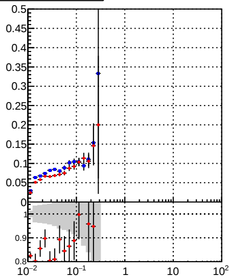
—•— /data2/legianni/BDT-vs-DNN/real-BDT/CMSSW_13_0_0_pre4/src/runrem/DQM_TT__mkFit_ —•— DQM_TT__mkFitRETEST_ Fake rate vs v
