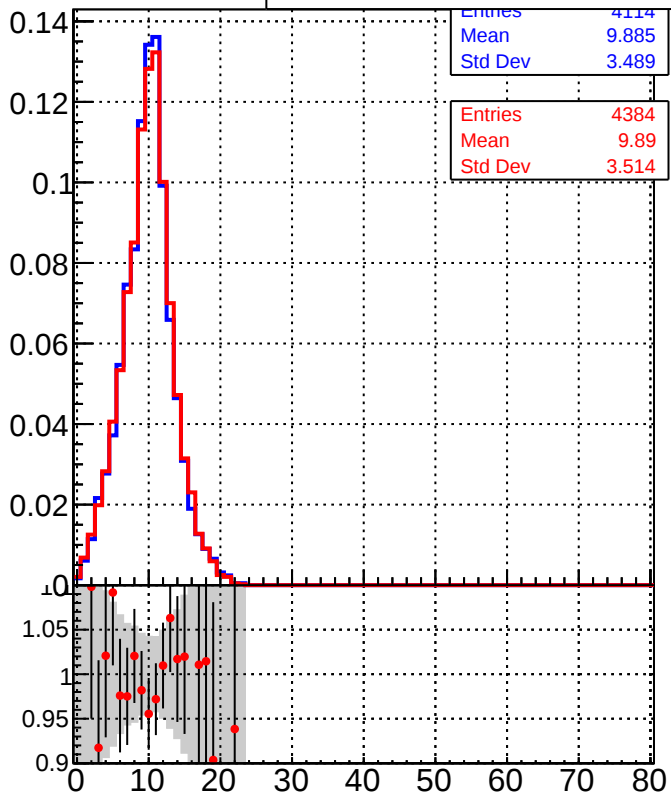
Legend: /data2/legianni/BDT-vs-DNN/real-BDT/CMSSW_13_0_0_pre4/src/runrem/DQM_TT_mkFit_ (blue line with squares), DQM_TT_mkFitRETEST_ (red line with circles)
