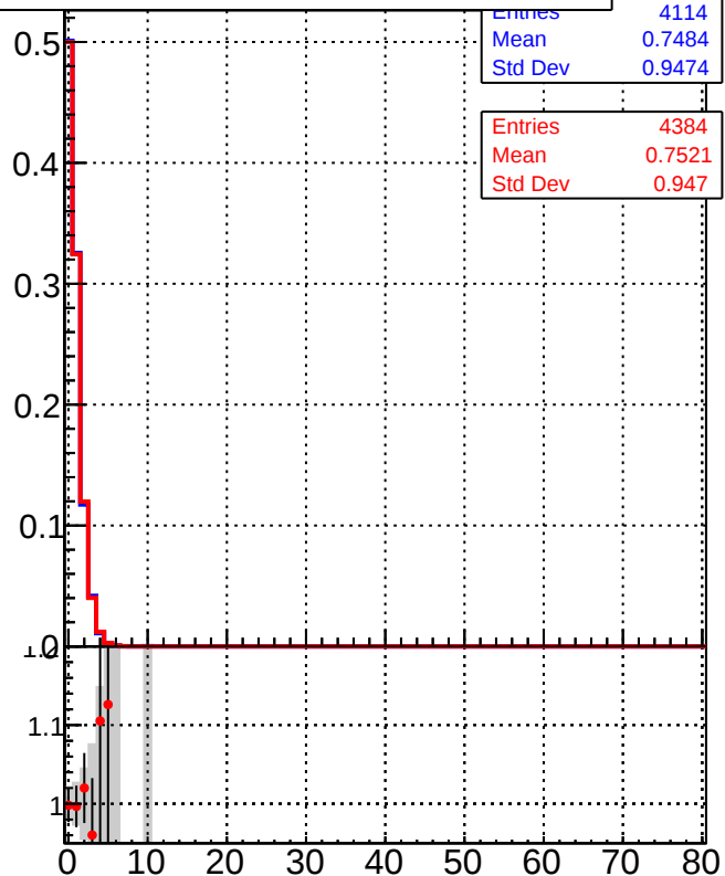
Legend: /data2/legianni/BDT-vs-DNN/real-BDT/CMSSW_13_0_0_pre4/src/runrem/DQM_TT_mkFit_ (blue line with squares), DQM_TT_mkFitRETEST_ (red line with circles)
