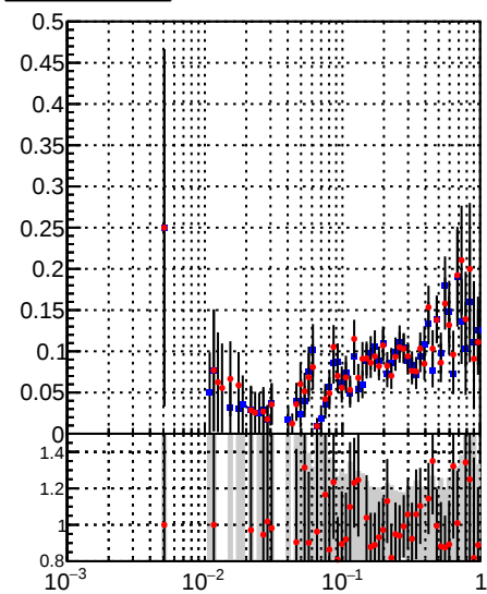
—•— /data2/legianni/BDT-vs-DNN/real-BDT/CMSSW_13_0_0_pre4/src/runrem/DQM_TT__mkFit_ —•— DQM_TT__mkFitRETEST_ Fake rate vs
