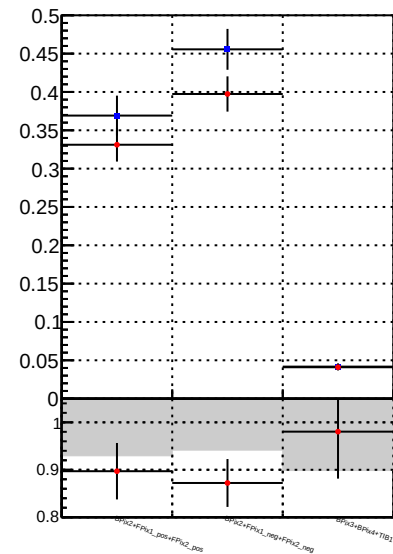
Fake rate vs. - /data2/legianni/BDT-vs-DNN/real-BDT/CMSSW_13_0_0_pre4/src/runrem/DQM_TT_mkFit_ - DQM_TT_mkFitRETEST
