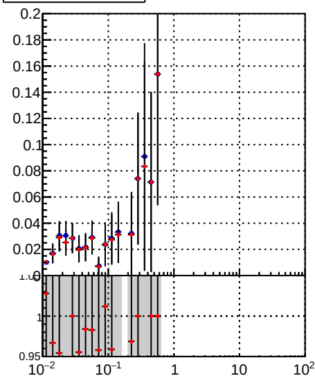
—●— /data2/legianni/BDT-vs-DNN/real-BDT/CMSSW_13_0_0_pre4/src/runrem/DQM_TT_mkFit_ —●— DQM_TT_mkFitRETEST_
