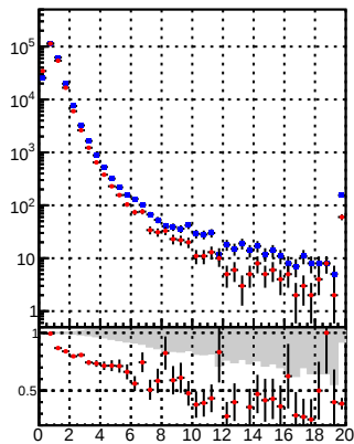
N of reco track vs. \chi^2 verSet
