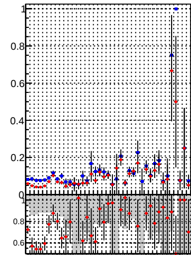
Fake rate vs. — /data2/legianni/BDT-vs-DNN/real-BDT/CMSSW_13_0_0_pre4/src/runrem/DQM_TT_mkFit_ — DQM_TT_mkFitRETEST
