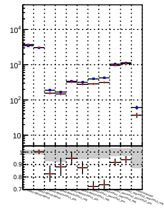
N of reco track vs. \chi^2 for \chi^2 bins
