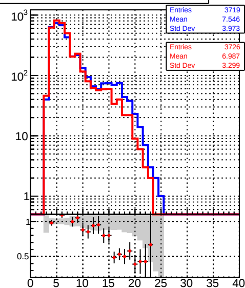
mean hit Legend: —•— /data2/legianni/BDT-vs-DNN/real-BDT/CMSSW_13_0_0_pre4/src/runrem/DQM_TT_mkFit_ —•— DQM_TT_mkFitRETEST_
