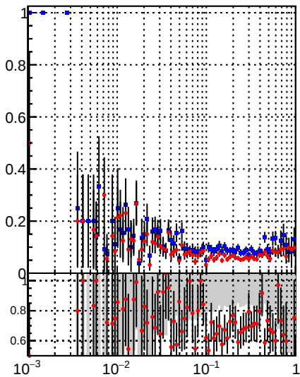
Fake rate vs —•— /data2/legianni/BDT-vs-DNN/real-BDT/CMSSW_13_0_0_pre4/src/runrem/DQM_TT__mkFit_ —•— DQM_TT__mkFitRETEST_
