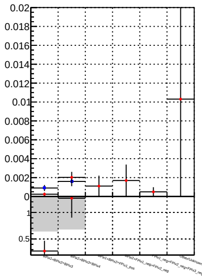
—●— /data2/legianni/BDT-vs-DNN/real-BDT/CMSSW_13_0_0_pre4/src/runrem/DQM_TT_mkFit_ —●— DQM_TT_mkFitRETEST
