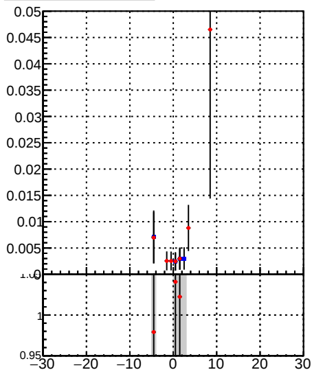
/data2/legianni/BDT-vs-DNN/real-BDT/CMSSW_13_0_0_pre4/src/runrem/DQM_TT_mkFit_ DQM_TT_mkFitRETEST
