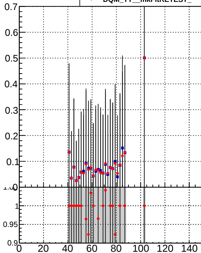
—■— /data2/legianni/BDT-vs-DNN/real-BDT/CMSSW_13_0_0_pre4/src/runrem/DQM_TT_mkFit_ —●— DQM_TT_mkFitRETEST_
