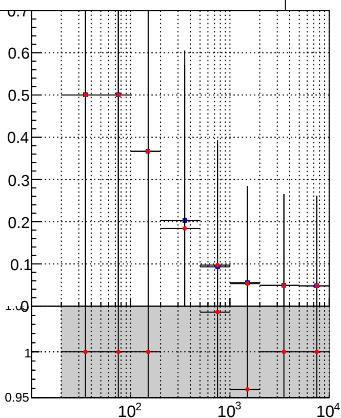
—■— /data2/legianni/BDT-vs-DNN/real-BDT/CMSSW_13_0_0_pre4/src/runrem/DQM_TT_mkFit_ —●— DQM_TT_mkFitRETEST_
