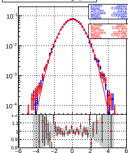
RecoAllAssoc2GenMatchedMerged_PulIX
