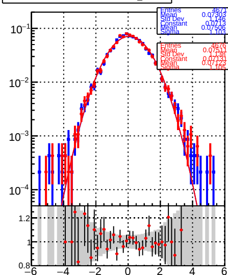
RecoPVAssoc2GenPVMatched_PulIX
