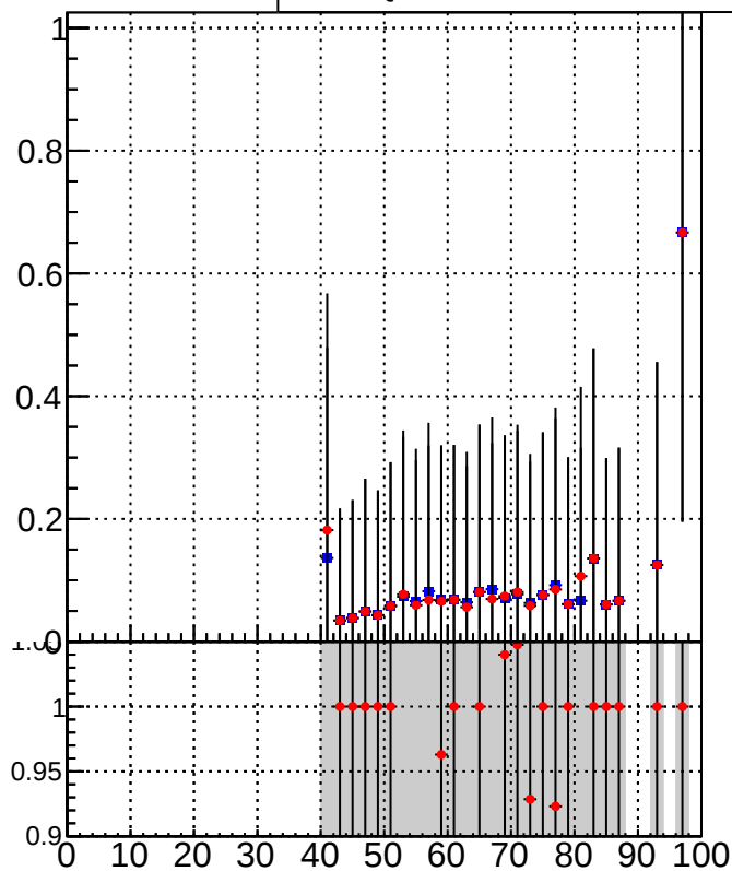
—■ /data2/legianni/BDT-vs-DNN/real-BDT/CMSSW_13_0_0_pre4/src/runrem/DQM_TT_mkFit_ —● DQM_TT_mkFitRETEST_
