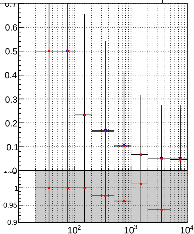
—■ /data2/legianni/BDT-vs-DNN/real-BDT/CMSSW_13_0_0_pre4/src/runrem/DQM_TT_mkFit_ —● DQM_TT_mkFitRETEST_
