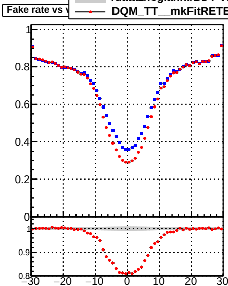
/data2/legianni/BDT-vs-DNN/real-BDT/CMSSW_13_0_0_pre4/src/runrem/DQM_TT_mkFit_ DQM_TT_mkFitRETEST_
