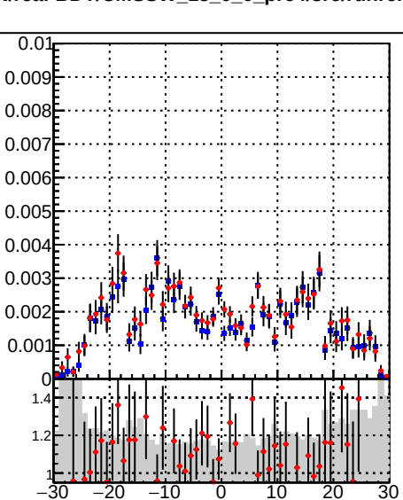
/data2/legianni/BDT-vs-DNN/real-BDT/CMSSW_13_0_0_pre4/src/runrem/DQM_TT_mkFit_ DQM_TT_mkFitRETEST_
