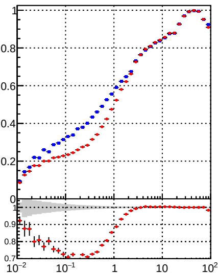
/data2/legianni/BDT-vs-DNN/real-BDT/CMSSW_13_0_0_pre4/src/runrem/DQM_TT_mkFit_ DQM_TT_mkFitRETEST_
