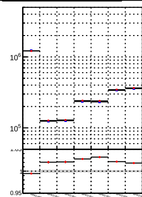
N of reco track vs. \chi^2 /data2/legianni/BDT-vs-DNN/real-BDT/CMSSW_13_0_0_pre4/src/runrem/DQM_TT_mkFit /data2/legianni/BDT-vs-DNN/real-BDT/CMSSW_13_0_0_pre4/src/runrem/DQM_TT_mkFitRETEST
