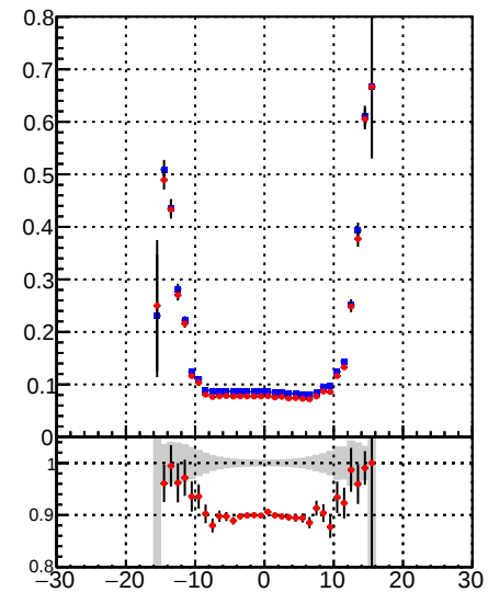
Fake rate vs d —●— /data2/legianni/BDT-vs-DNN/real-BDT/CMSSW_13_0_0_pre4/src/runrem/DQM_TT_mkFit_ —●— DQM_TT_mkFitRETEST
