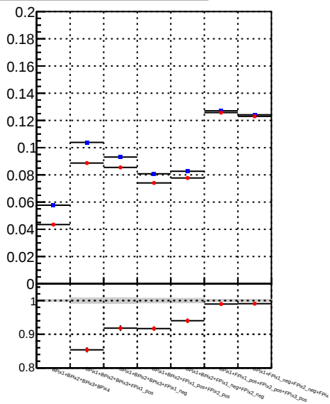
Fake rate vs. — /data2/legianni/BDT-vs-DNN/real-BDT/CMSSW_13_0_0_pre4/src/runrem/DQM_TT_mkFit_ — DQM_TT_mkFitRETEST
