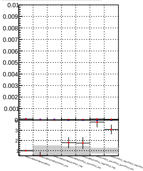
Fake rate vs. — /data2/legianni/BDT-vs-DNN/real-BDT/CMSSW_13_0_0_pre4/src/runrem/DQM_TT_mkFit_ — DQM_TT_mkFitRETEST
