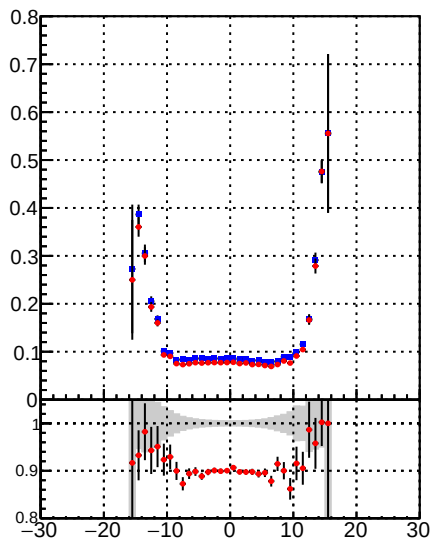
—●— /data2/legianni/BDT-vs-DNN/real-BDT/CMSSW_13_0_0_pre4/src/runrem/DQM_TT_mkFit_ —●— DQM_TT_mkFitRETEST
