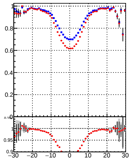
—●— /data2/legianni/BDT-vs-DNN/real-BDT/CMSSW_13_0_0_pre4/src/runrem/DQM_TT_mkFit_ —●— DQM_TT_mkFitRETEST
