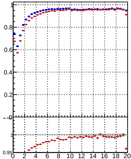
—●— /data2/legianni/BDT-vs-DNN/real-BDT/CMSSW_13_0_0_pre4/src/runrem/DQM_TT_mkFit_ —◆— DQM_TT_mkFitRETEST
