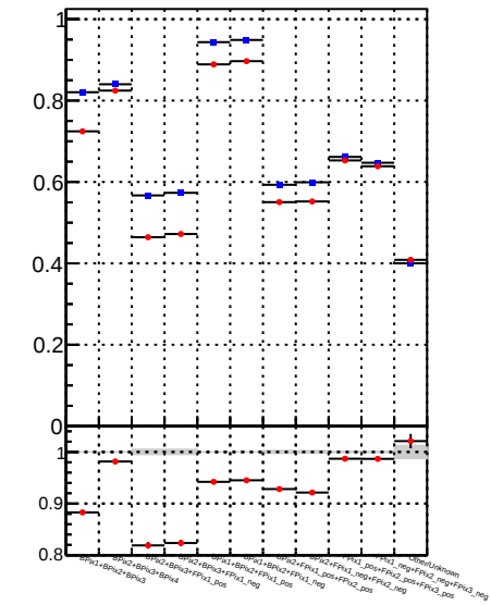
—●— /data2/legianni/BDT-vs-DNN/real-BDT/CMSSW_13_0_0_pre4/src/runrem/DQM_TT_mkFit_ —◆— DQM_TT_mkFitRETEST
