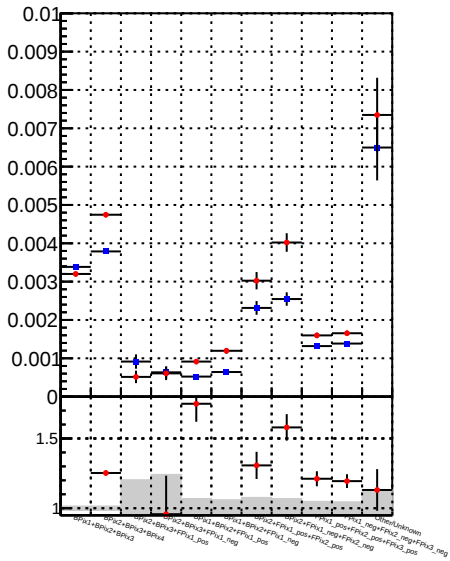
—●— /data2/legianni/BDT-vs-DNN/real-BDT/CMSSW_13_0_0_pre4/src/runrem/DQM_TT_mkFit_ —◆— DQM_TT_mkFitRETEST
