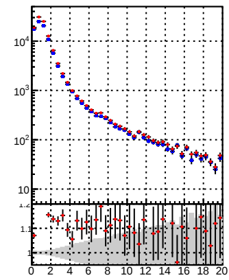
N of reco track vs. \chi^2 for \chi^2 bins
