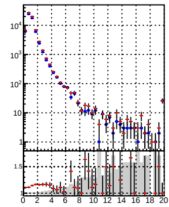
N of reco track vs. \chi^2 verSet
