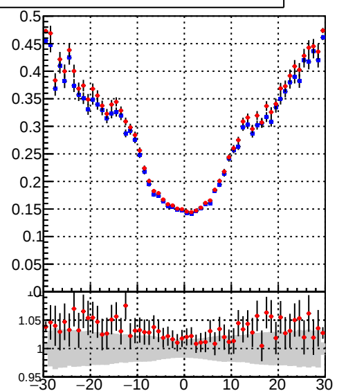
—•— /data2/legianni/BDT-vs-DNN/real-BDT/CMSSW_13_0_0_pre4/src/runrem/DQM_TT_mkFit_ —•— DQM_TT_mkFitRETEST_
