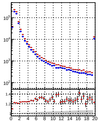
N of reco track vs. \chi^2 - /data2/legianni/BDT-vs-DNN/real-BDT/CMSSW_13_0_0_pre4/src/runrem/DQM_TT_mkFit - DQM_TT_mkFitRETEST
