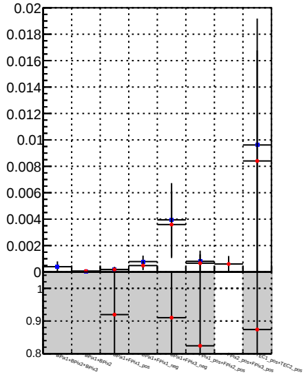
Fake rate vs. —•— /data2/legianni/BDT-vs-DNN/real-BDT/CMSSW_13_0_0_pre4/src/runrem/DQM_TT_mkFit_ -x- DQM_TT_mkFitRETEST
