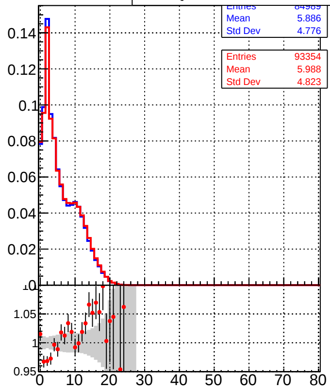
/data2/legianni/BDT-vs-DNN/real-BDT/CMSSW_13_0_0_pre4/src/runrem/DQM_TT_mkFit_ DQM_TT_mkFitRETEST_
